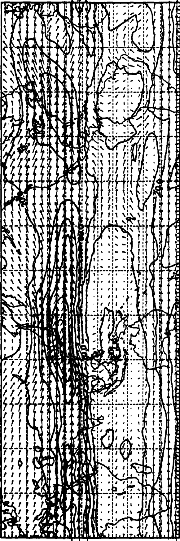
OBSERVED WIND 200MB WIN 1980
